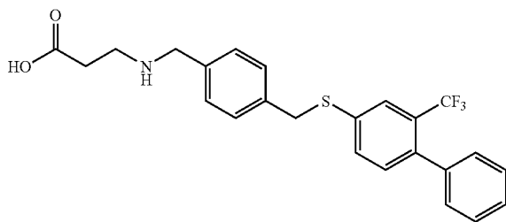
3-[4-(2-trifluoromethyl-biphenyl-4-ylsulfanylmethyl)-benzylamino]-propionic acid
