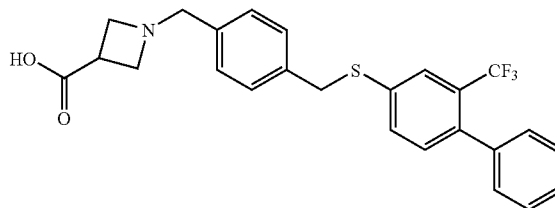
1-[4-(2-Trifluoromethyl-biphenyl-4-ylsulfanylmethyl)-benzyl]-azetidone-3-carboxylic acid
